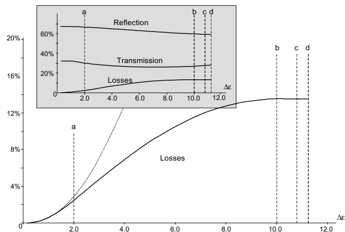
Figure 2: Out-of-plane scattering losses for a single air slot.
