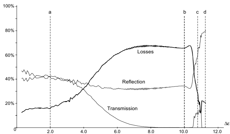
Figure 4: Reflection, Transmission and out-of-plane scattering loss averaged over a structure with 30 to 50 periods.
