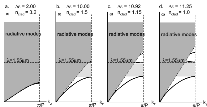
Figure 3: Band structures of the structure in figure 1 for different \Delta\epsilon .
