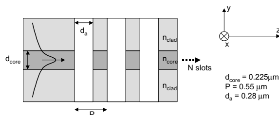
Figure 1: The simulated structure. A symmetric 3 layer slab waveguide periodically intersected with air slots
