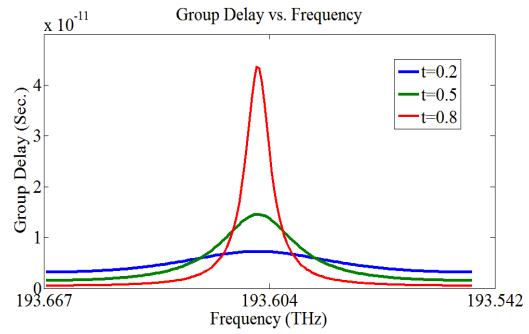
Fig. 2. The group delay response for single MRRs
