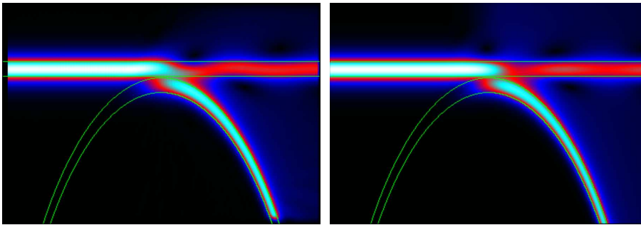
Figure 3: The absolute value field plots of FDTD (left) and CMT (right) calculations of the structure defined in Figure 2.
