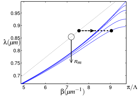
Figure 2: Dispersion curves for the considered model structure for n_m = 0 (dotted) and n_m = 0.01, 0.05, 0.1, 0.2, and 0.3 , with d_1 = d_2 = 0.1613 \mu\text{m} , n_{av} = 1.55 .
