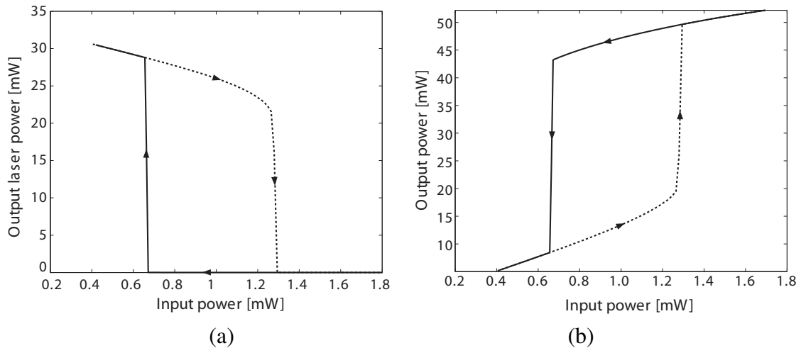
Figure 2: Simulation results of the bistable behavior of a \lambda/4 -shifted and AR-coated multiquantum well DFB-laser with length 400 \mu\text{m} , \kappa L 1.2 and active layer thickness 40 nm. The laser is electrically pumped with I/I_{th} = 4 and I_{th} = 42.5 \text{ mA} . a) Laser output power as a function of the power of the injected light; b) Amplification of the injected light
