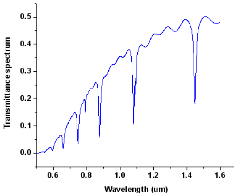
Fig. 2. Transmittance spectrum of the sensor with a refractive index of liquid of 1.33.
