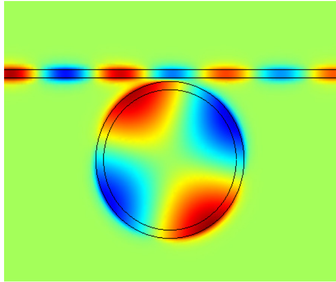
Fig. 3. Field distribution in the plasmonic ring resonator based sensor C at the resonance wavelength \lambda=1.448 \mu\text{m} .
