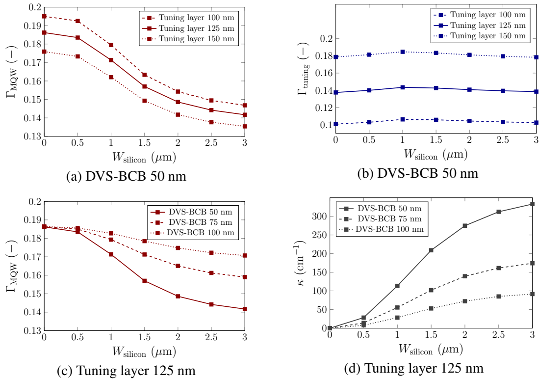
Figure 2: Fundamental mode confinement factors dependence on DVS-BCB thickness, tuning layer thickness and silicon waveguide width.
