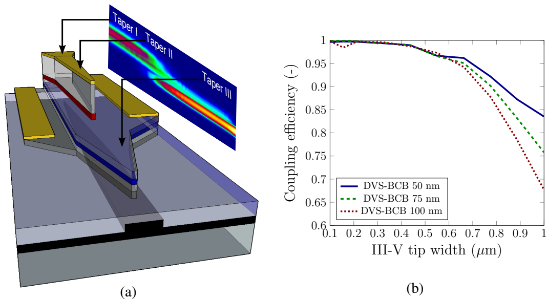
Figure 3: Adiabatic tapered III-V/SOI coupler. (a) Schematic; (b) Influence of the III-V tip width on the coupling efficiency.
