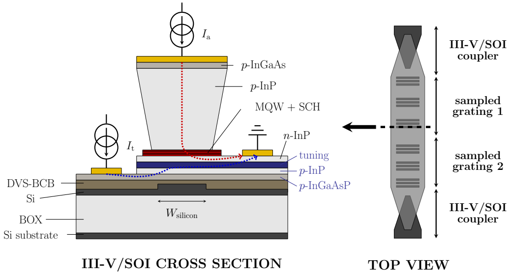
Figure 1: Layout of the proposed III-V/SOI TTG laser diode. I_a and I_t represent the active and tuning current respectively.
