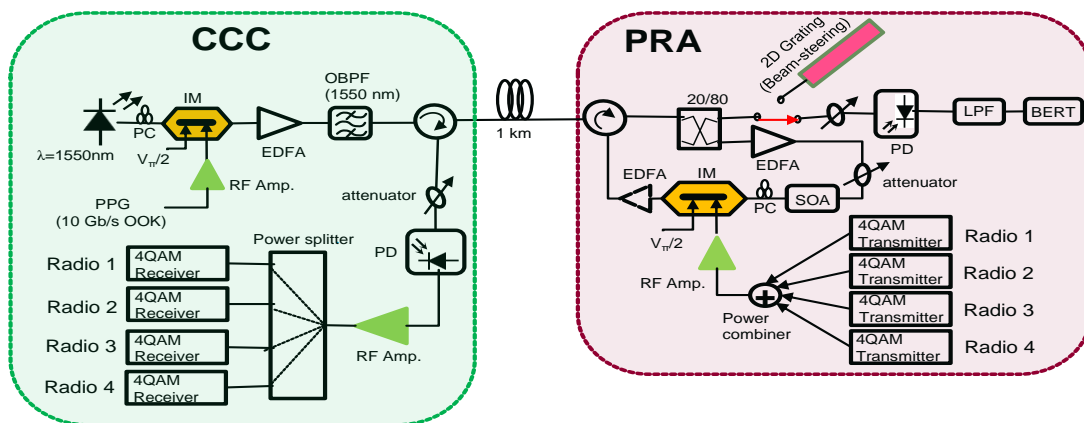
Fig. 2 Simulation setup
