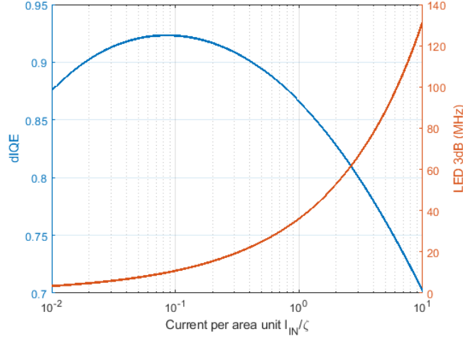
Fig. 1: Differential (small signal) efficiency dIQE and the f_{3dB} versus the current per unit area. Higher current density accelerates (higher f_{3dB} ), but reduces the efficiency.
